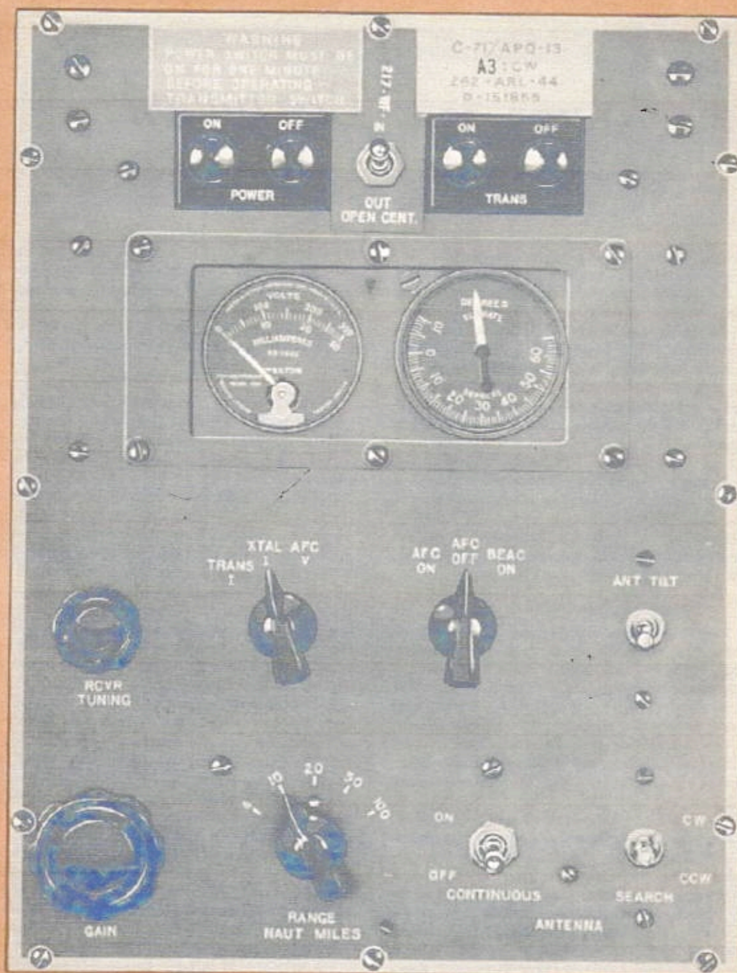
MAIN CONTROL BOX
